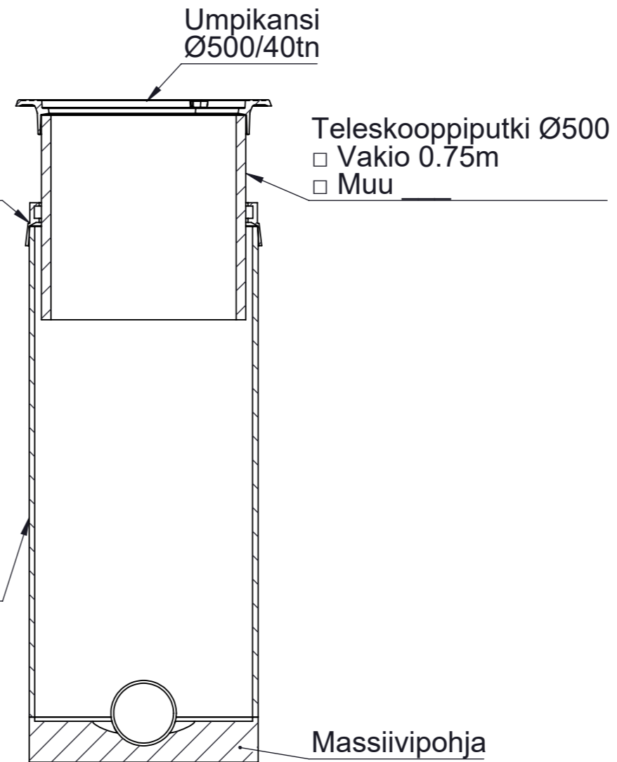
SECTION C-C SCALE 1 : 13
